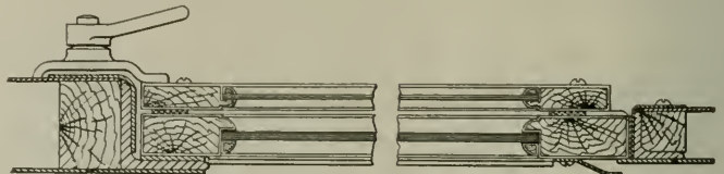
DETAILED SECTION OF SHEATHED WINDOW SASH.
